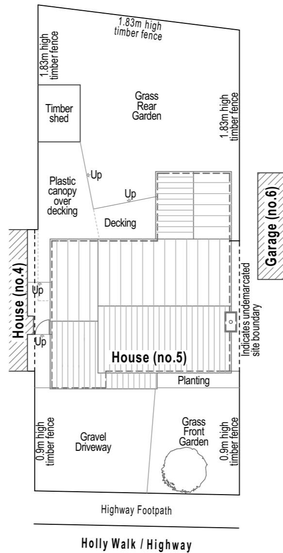
Proposed Site Layout Plan 1:200
